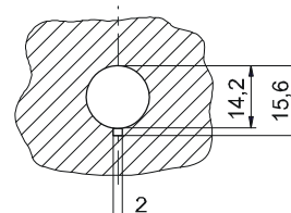
Mounting hole at burner chassis
